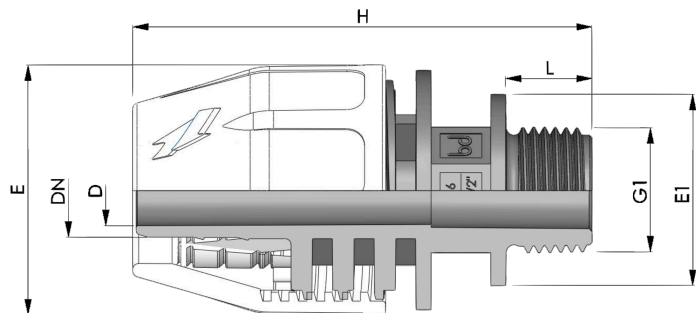
Straight Fitting
